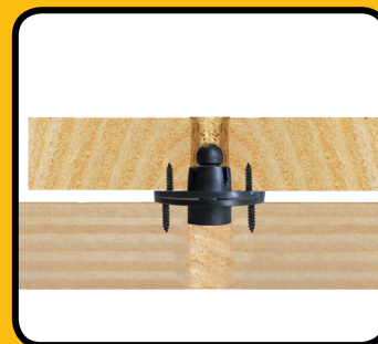
STEP 3: Snap together
